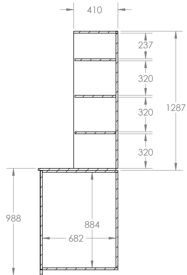
SECTION E-E
